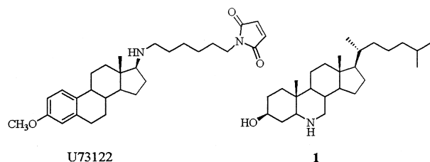
Figure 1. Chemical structures of U73122 and compound 1 .
